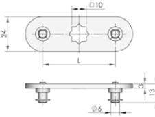
Optional cam S2C2500 S2C2000
