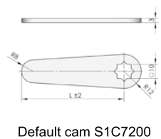
Default cam S1C7200
